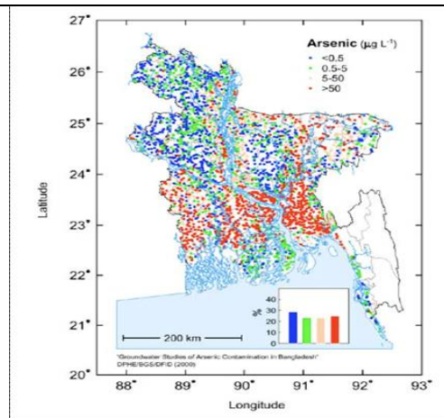
DPHE/BGS/DFID (2000): Gov. of Bangladesh. Recent maps show severe contamination throughout the Ganga-Meghna-Brahmaputra basin.
