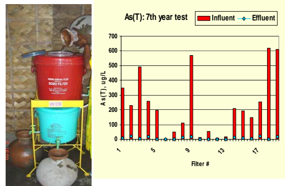
Test results compiled over seven years show SONO can remove arsenic (to < 10 ppb), manganese (a neurotoxin to < 400 ppb)), iron, and all transition metal ions to a safe potable water.
